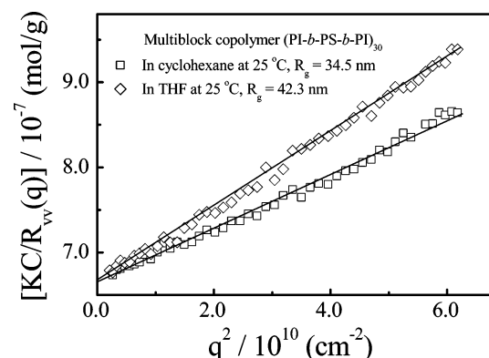
Figure 12. Angular dependence of Rayleigh ratio KC/R_w(q) of narrowly distributed multiblock copolymer (PI- b -PS- b -PI) 30 chains in a good solvent (THF) and in a selective solvent (cyclohexane, a poor solvent for the PS block at 25 °C).
