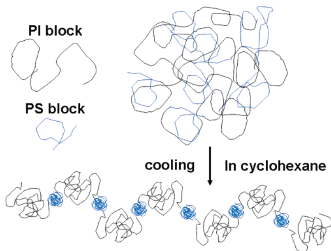
Figure 15. Schematic of conformation change of a multiblock (PI- b -PS- b -PI) n chain in cyclohexane, a solvent selectively poor for the PS block at lower temperatures, as the solution temperature decreases.
