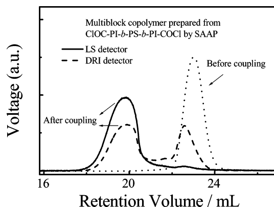
Figure 9. SEC profiles of triblock \alpha,\omega -diacyl chloride CIOC-PI- b -PS- b -PI-COCl chains after the coupling in n -hexane with the assistant of the self-assembly.
