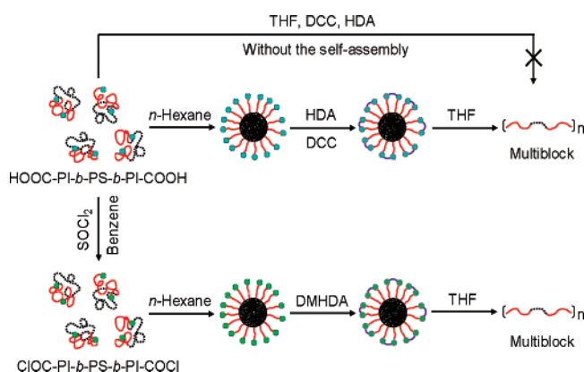
Figure 2. Schematic of coupling PI- b -PS- b -PI triblock copolymer chains with two active end in a solvent selectively good for PI (self-assembly assisted polypolymerization, SAAP) and in a good solvent for both PS and PI (no self-assembly).
